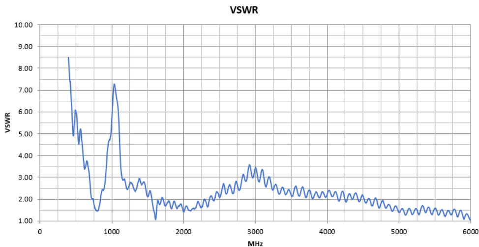
Figure 2. VSWR graph
